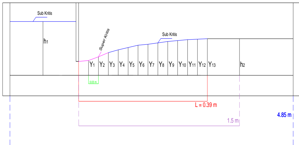
Gambar 4 Profil Loncat air Q = 0.002 \text{ m}^3/\text{dtk} dan W = 0.030 \text{ m}
