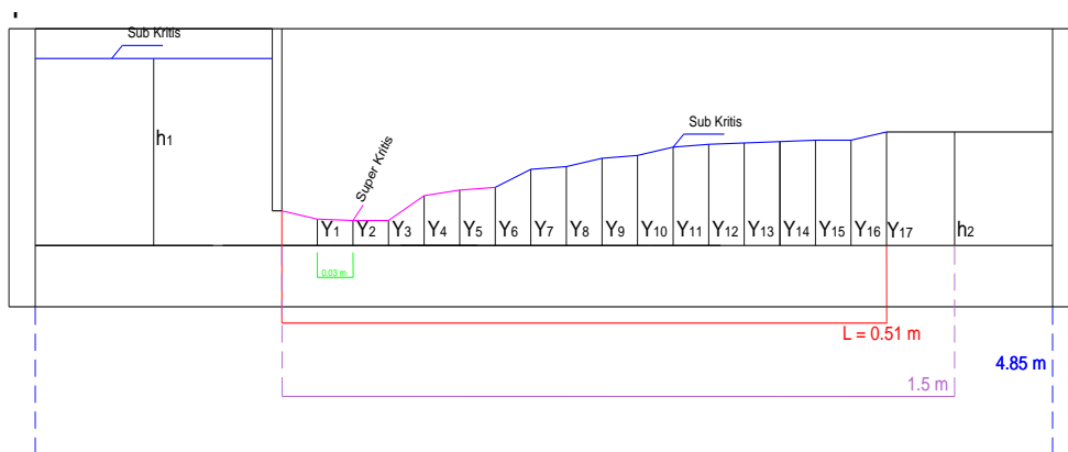
Gambar 2 Profil Loncat air Q = 0.002 \text{ m}^3/\text{dtk} dan W = 0.025 \text{ m}
