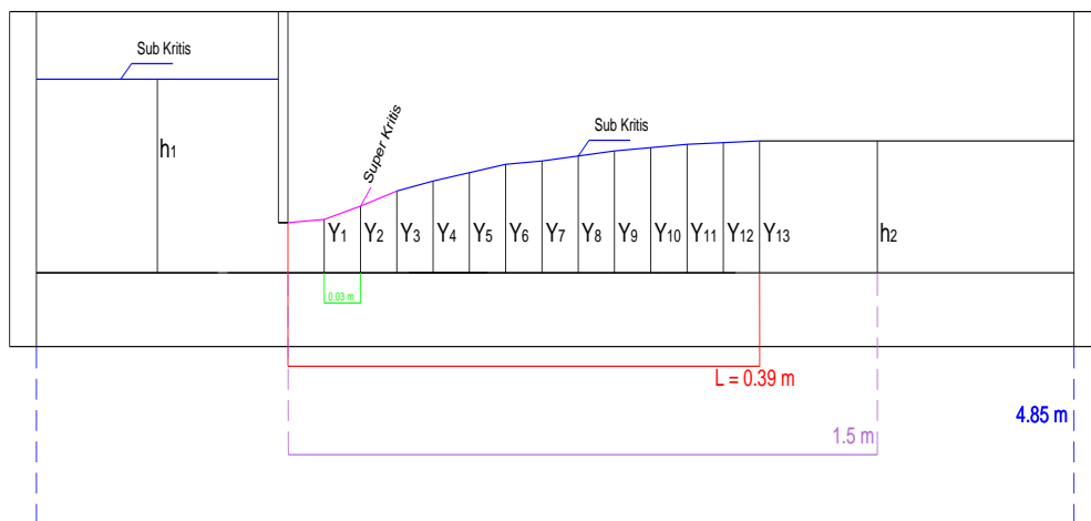
Gambar 3 Profil Loncat air Q = 0.002 \text{ m}^3/\text{dtk} dan W = 0.028 \text{ m}
