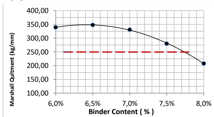
Gambar 5 Hubungan kadar aspal vs Marshall Quotient
