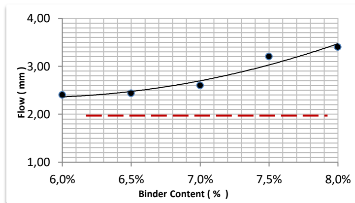
Gambar 4 Hubungan kadar aspal vs flow
